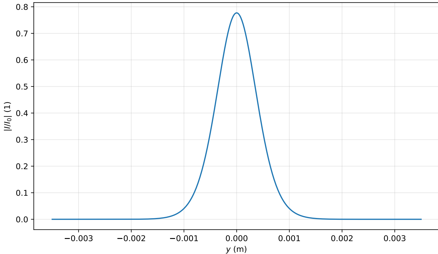
Intensity profile I(x=0, y, z=1.831)/I_0 , P_{in}=0.4P_{cr} , artificial time
